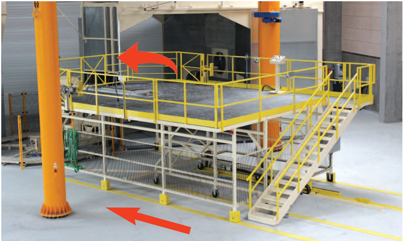
Shown above is a single-station traveling platform in position to service the arm with the roll-over safety fence indexed forward.
